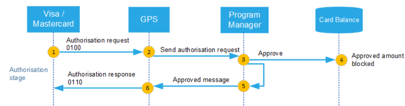
Figure: Authorisation Flow - Approve
