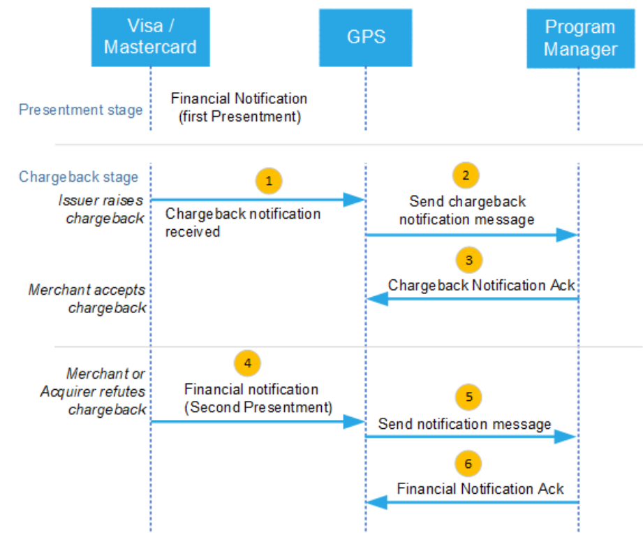
Figure: ChargebackTransaction Flow
