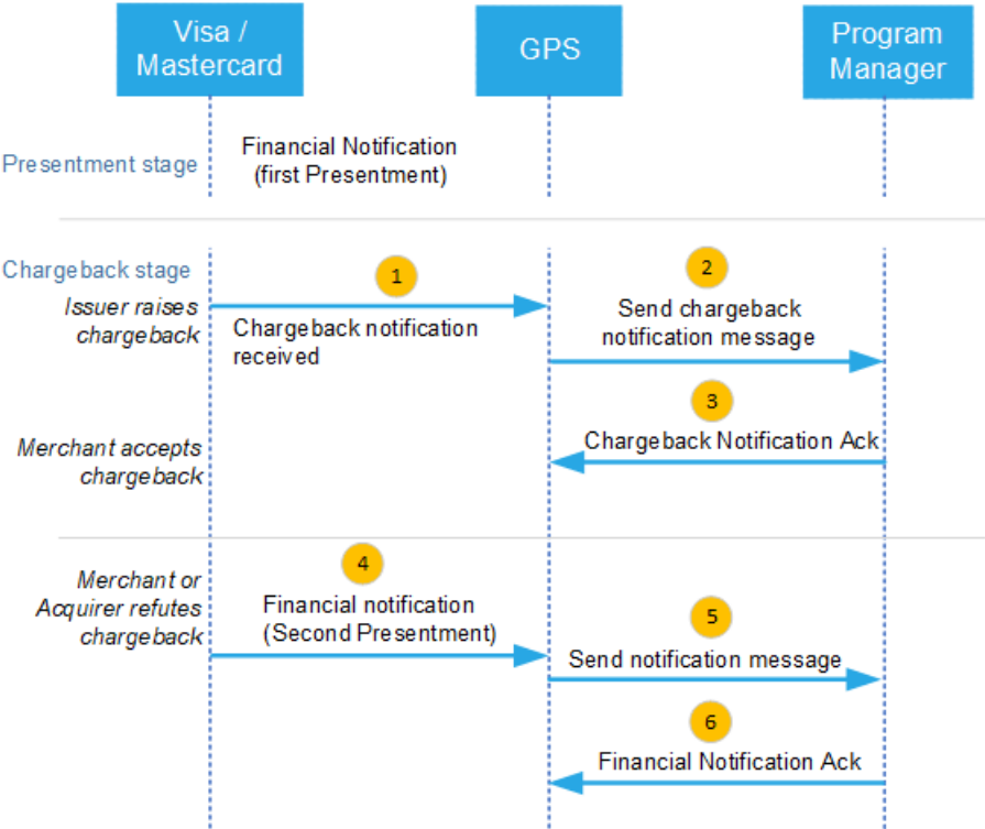
Figure 16: ChargebackTransaction Flow
