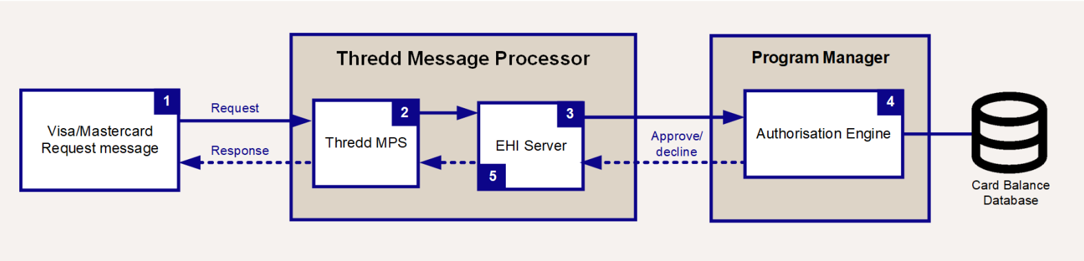
Figure 2: EHI Mode 1 - external host approves transaction
