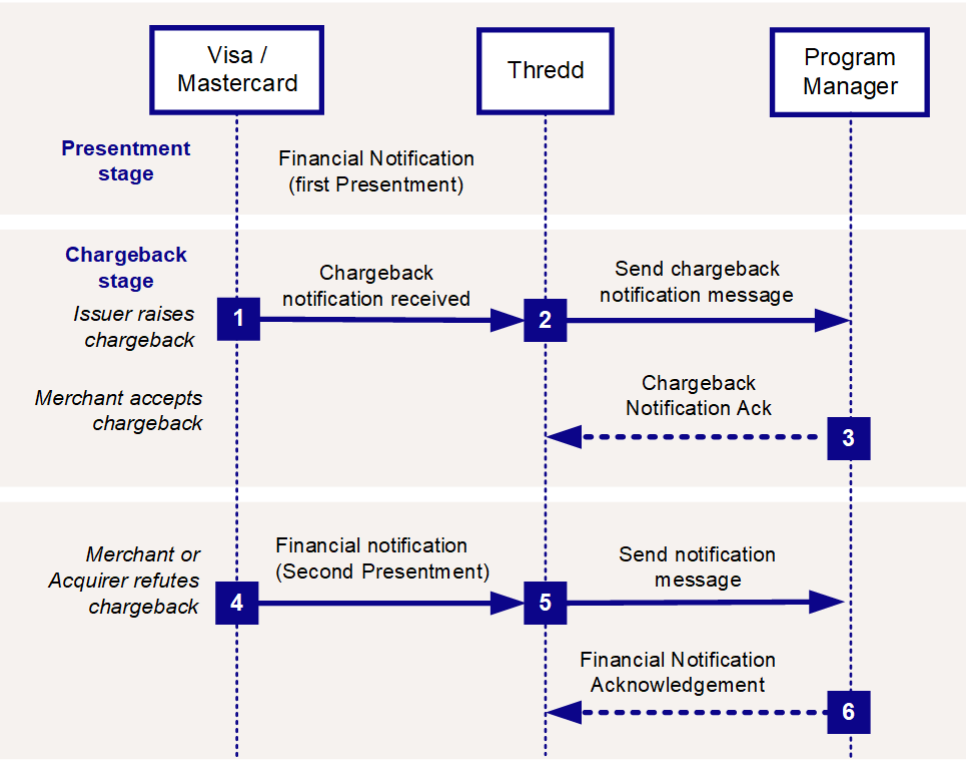
Figure 16: ChargebackTransaction Flow
