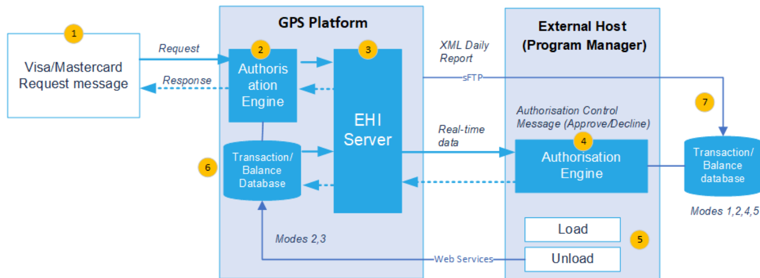
GPS System Components and External Host Interface Message Flow
