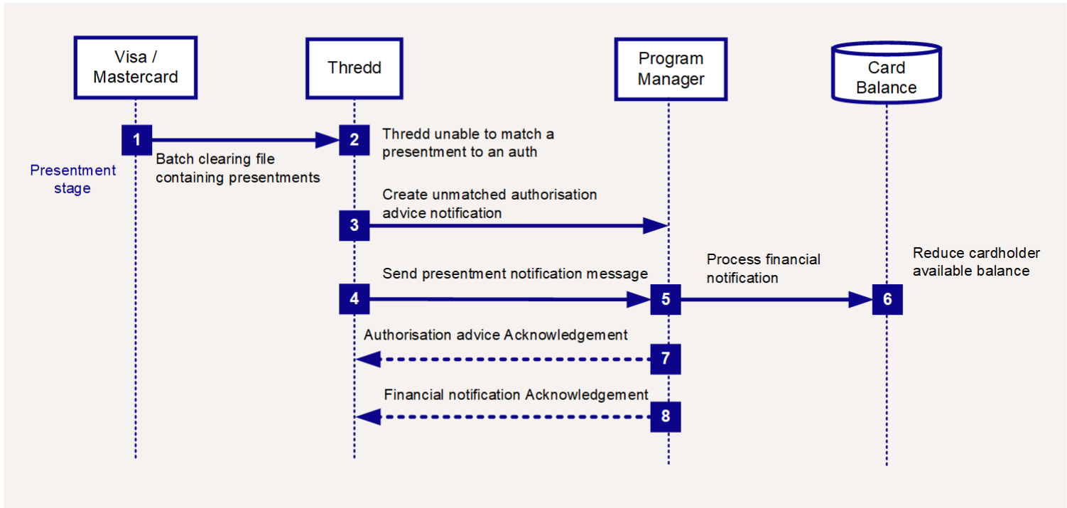
Figure 15: Offline Transaction - Presentment Flow
