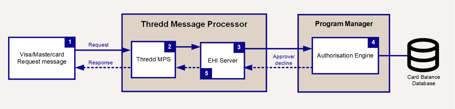
Figure 3: Gateway Processing (Mode 1) - external host approves transaction
