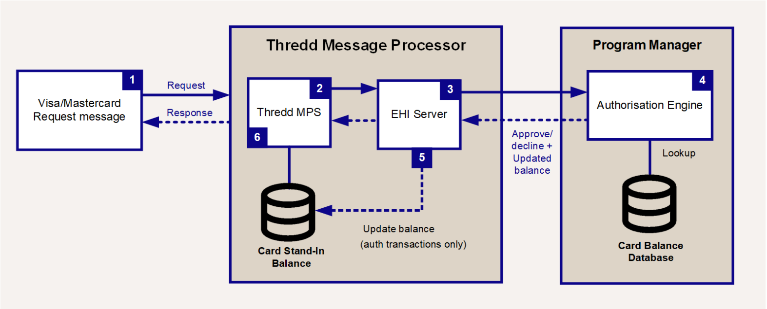
Figure 7: Gateway Processing with STIP (Mode 5) - External host authorises, but Thredd can approve if the external host is not available
