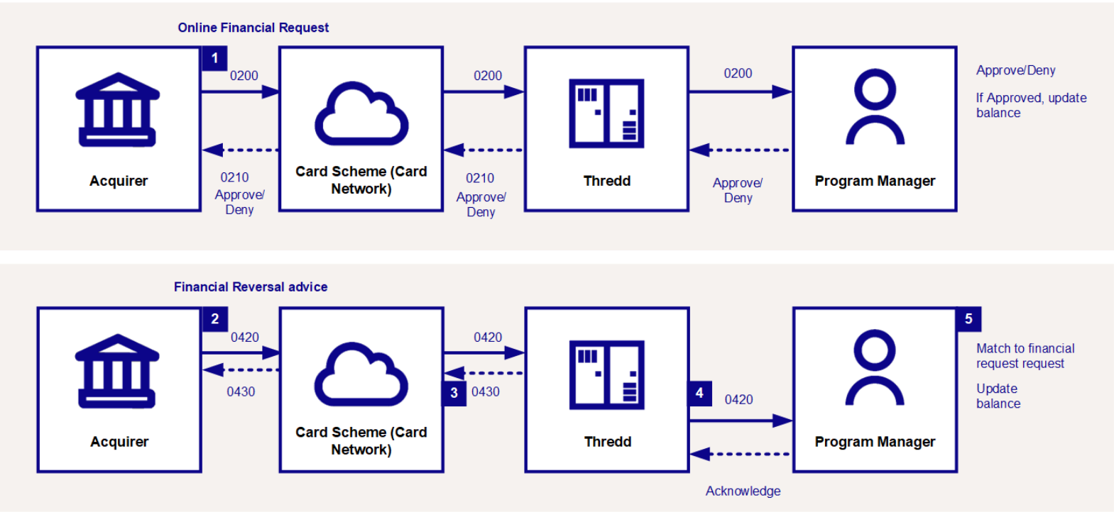
Figure 15: Authorisation Reversal Flow
