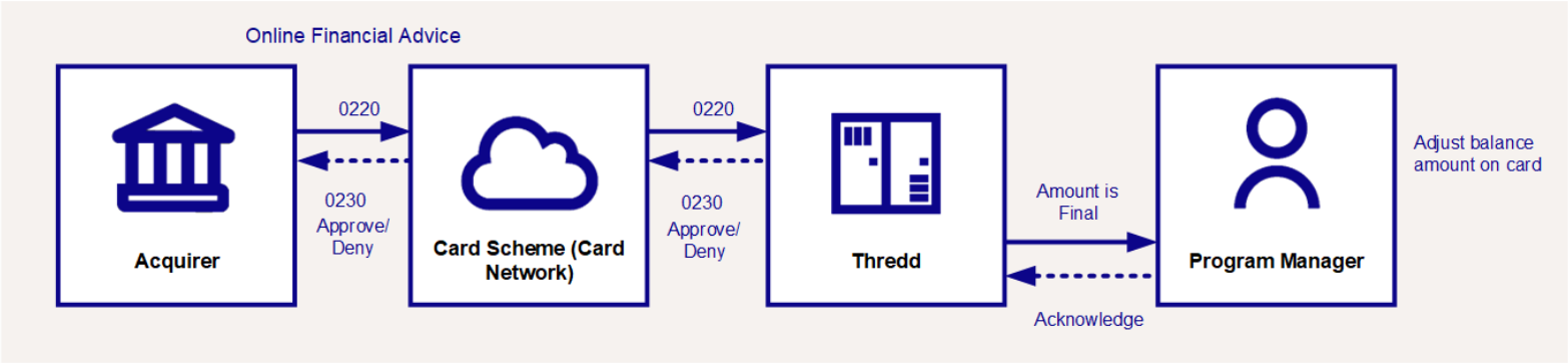
Figure 16: Financial Advice Flow
