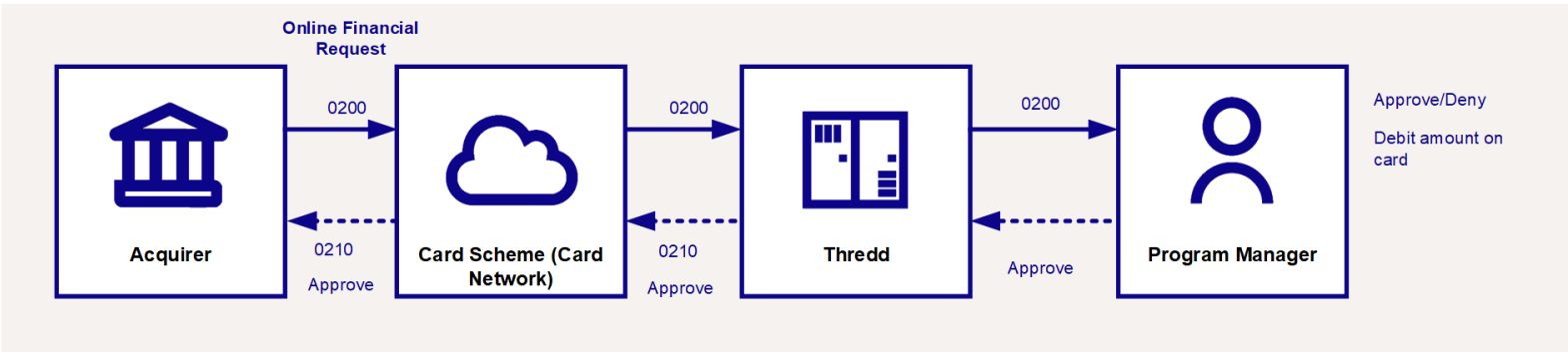
Figure 13: Financial Authorisation Flow - Approve
