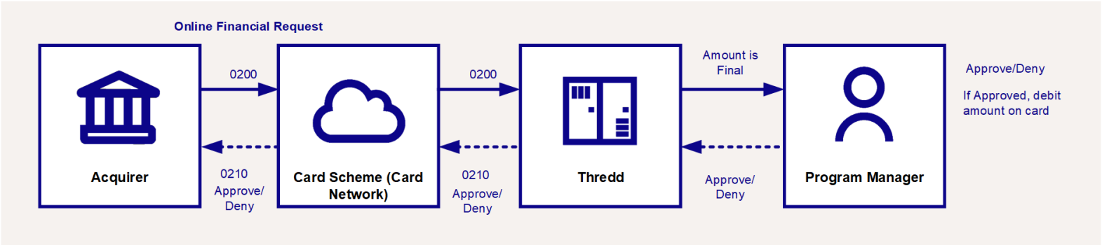
Figure 12: Single Message System
