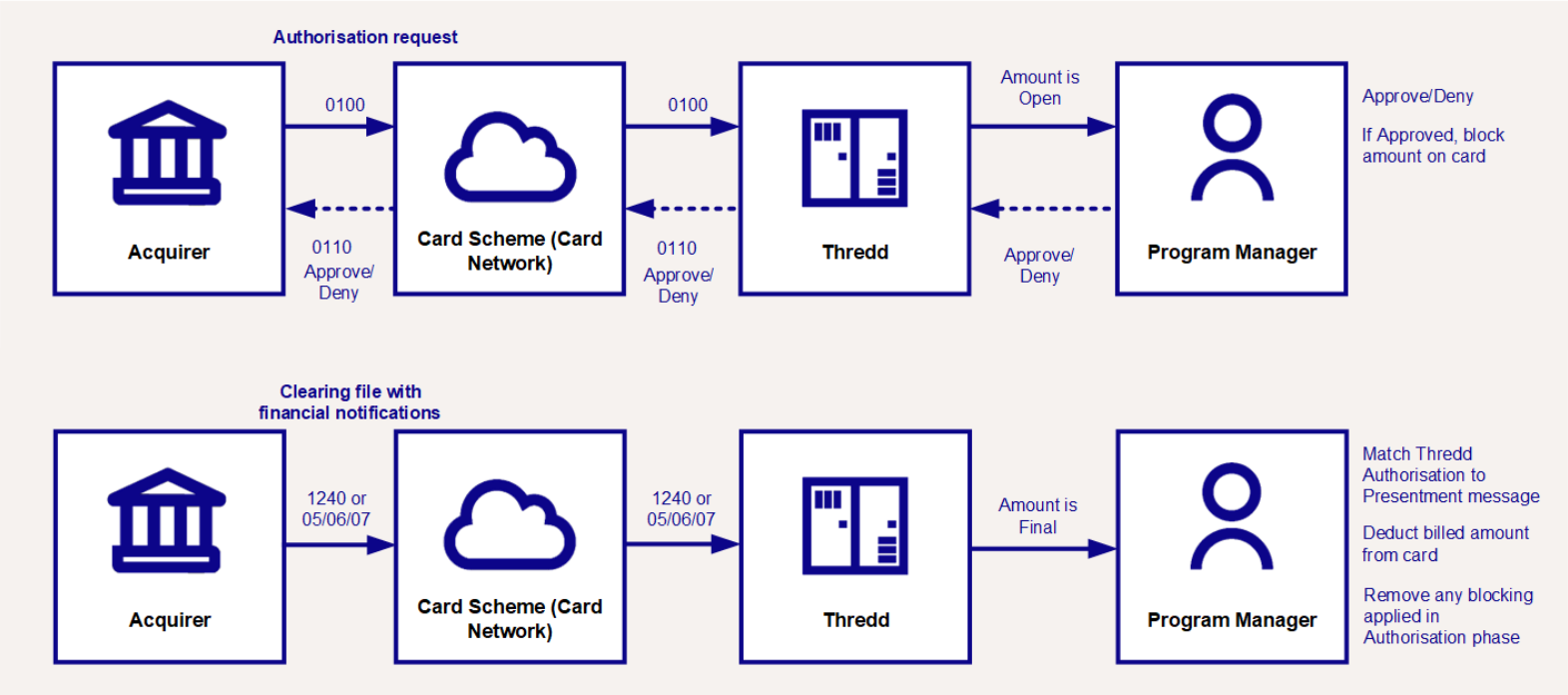
Figure 11: Dual Message System
