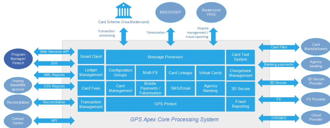
Figure 4-1: GPS System Architecture
