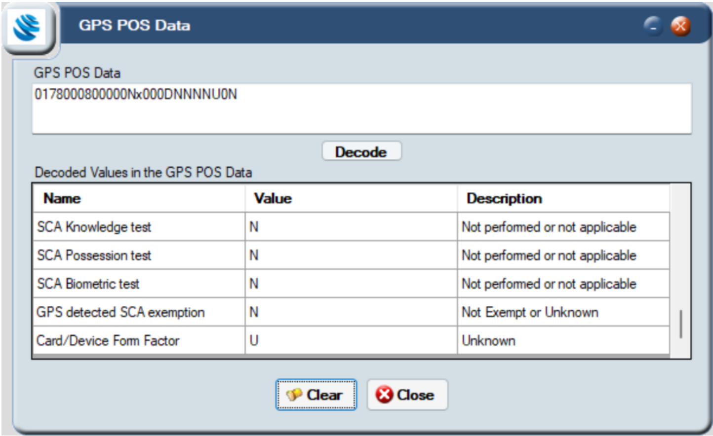
Figure 9: GPS POS Data in Smart Client showing some of the SCA information
