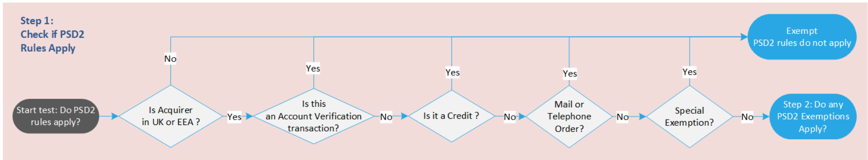
Figure 4: PSD2 Check Step 1: Exempt from PSD2 Rules
