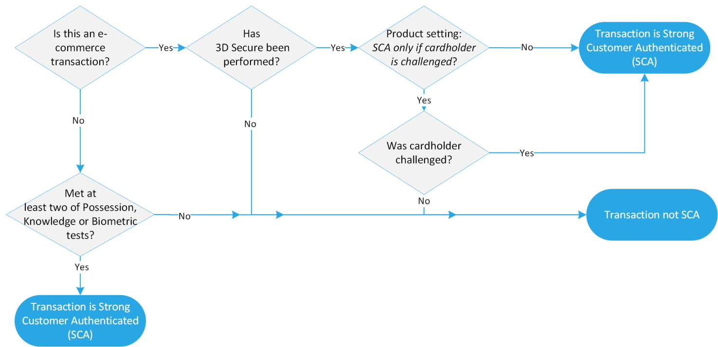
Figure 2: Strong Customer Authentication (SCA) Checks
