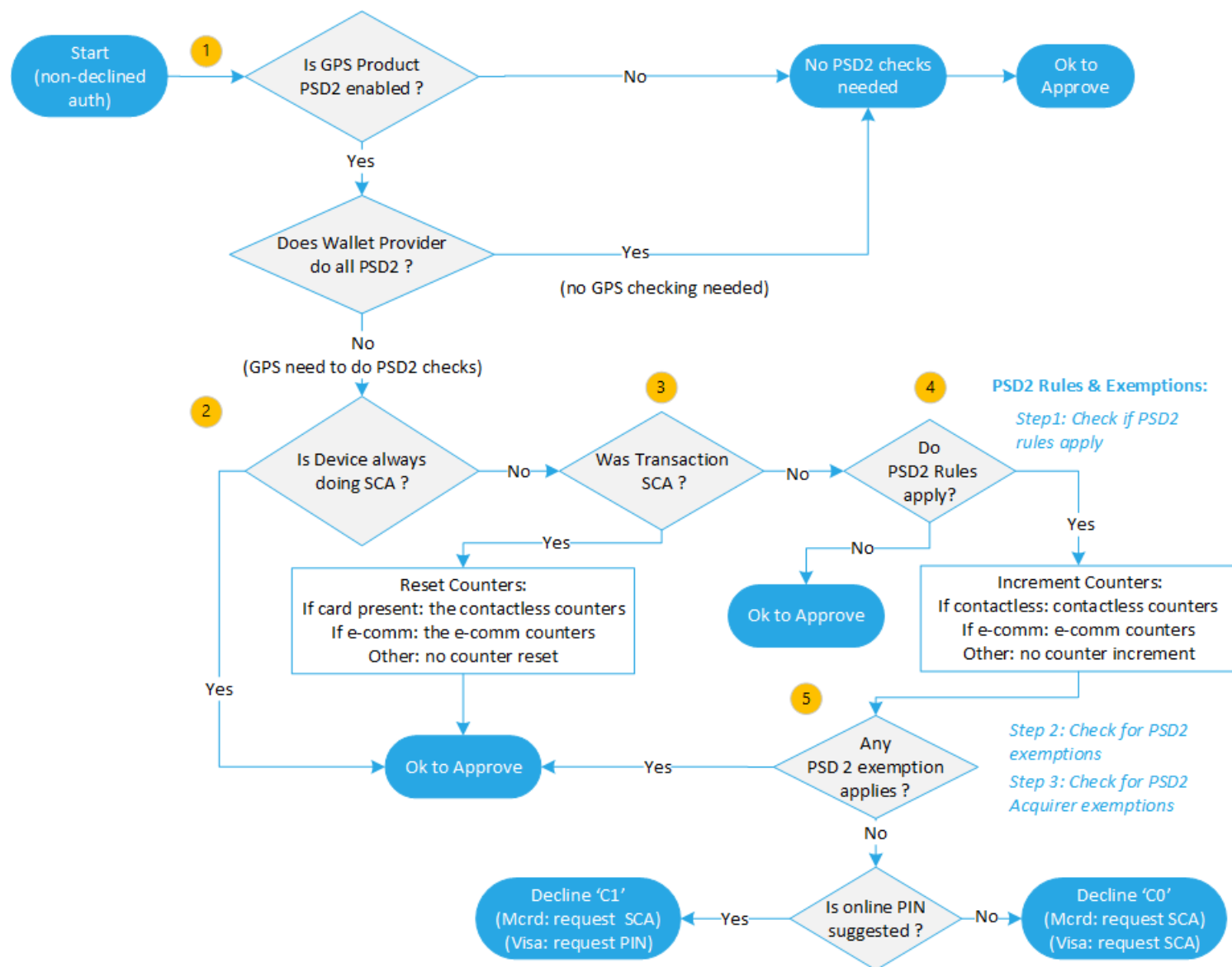
Figure 1: Transaction Checks under PSD2 (for Payment Authorisation)
