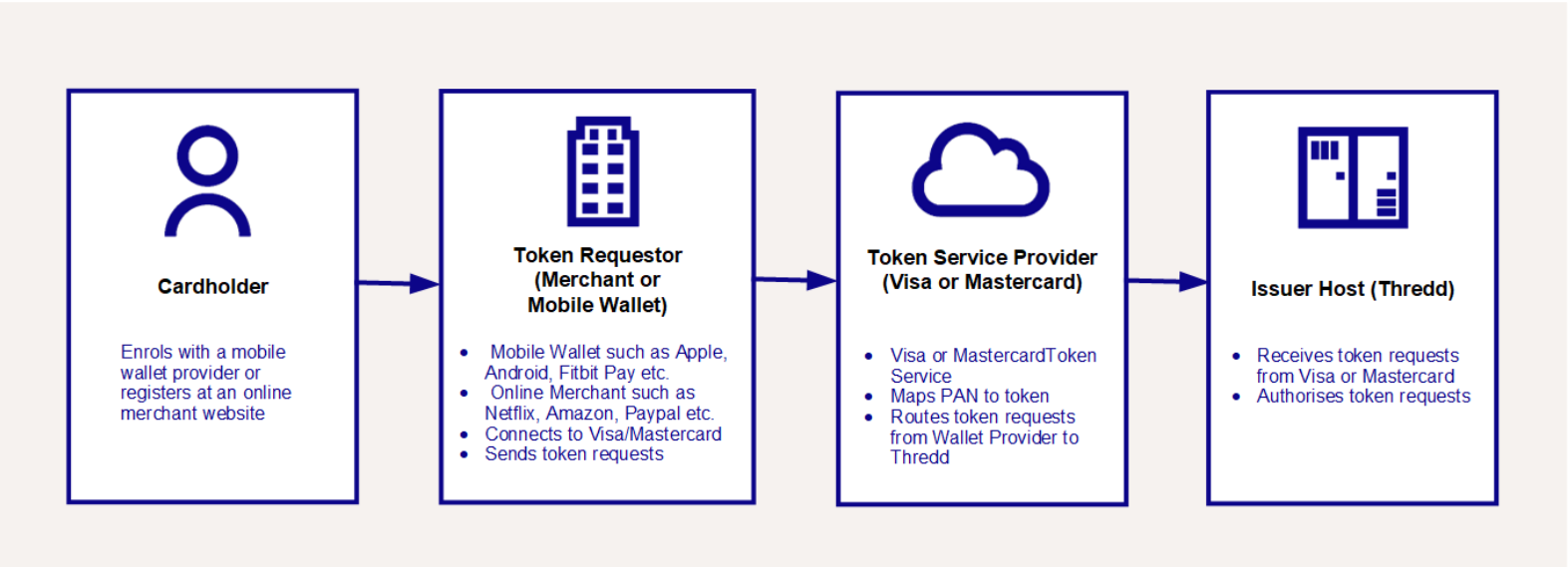
Figure 54: Parties involved in the MDES/VDEP tokenisation flow
