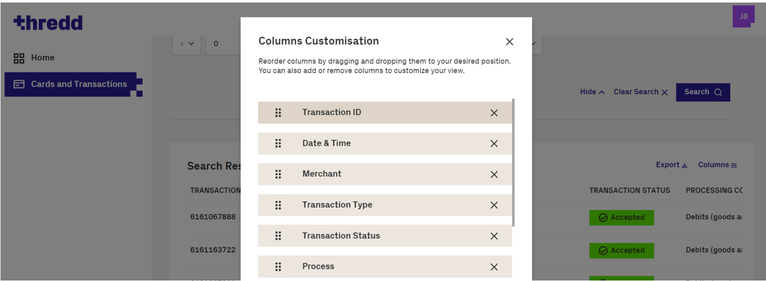
Figure 29: Columns Customisation
