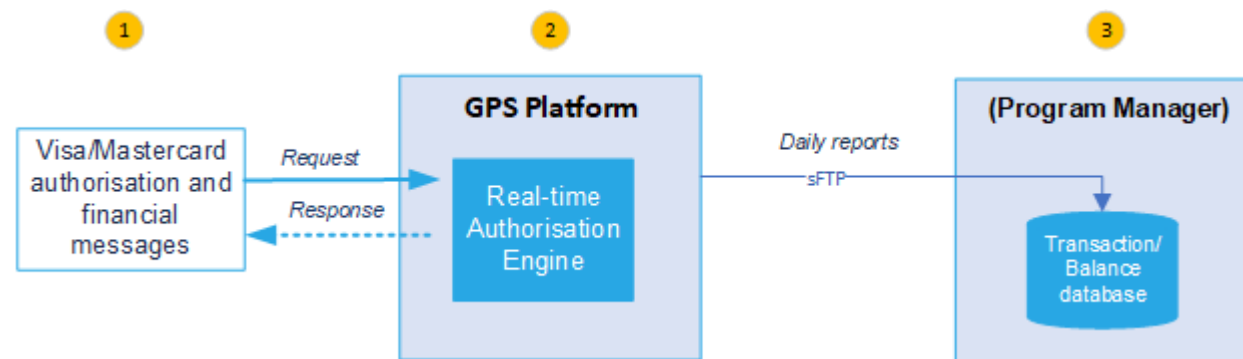
Figure 1: XML Reporting
