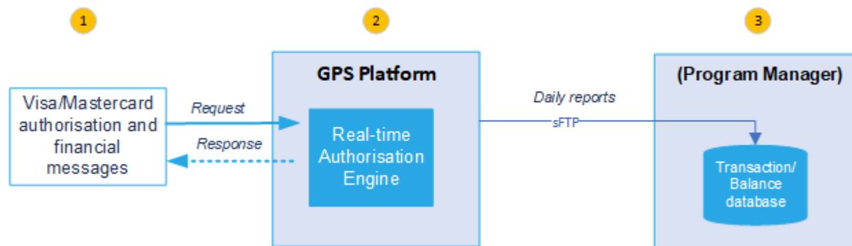
Figure 1: XML Reporting
